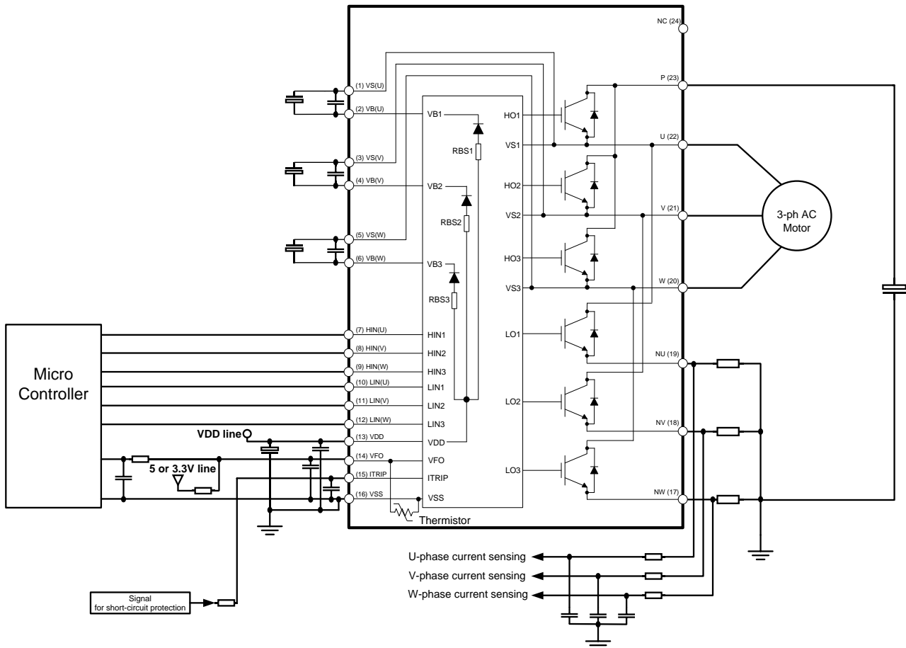
Figure 9: Application circuit
